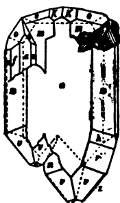
Canaan, Conn.
