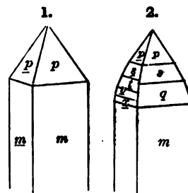
Greenland, Knr.
