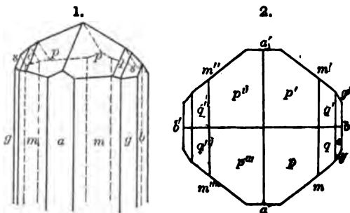
Branchville, Conn.
