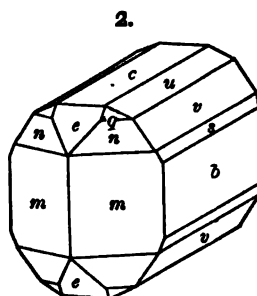
Figs. 1-3, Stoneham.
