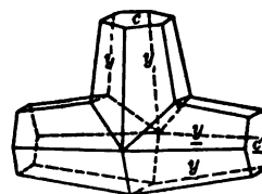
Elizabethtown 4 .
