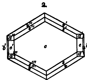
Sternbergite, Haid.
