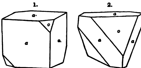
Figs. 1, 2, Utah, Pearce.
