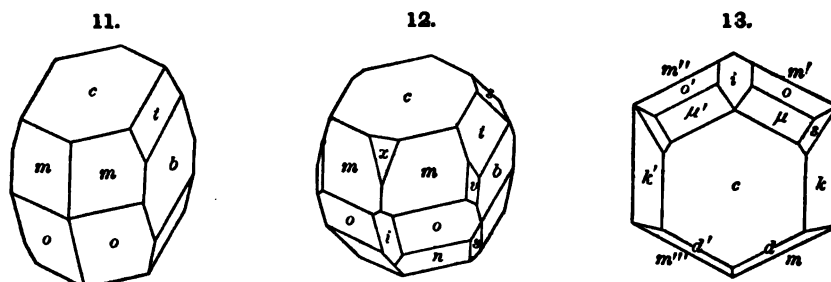
Figs. 11–13, Achmatovsk, Kk.
