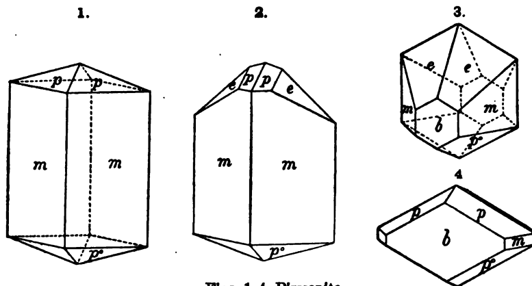
Figs. 1-4, Pirssonite.
