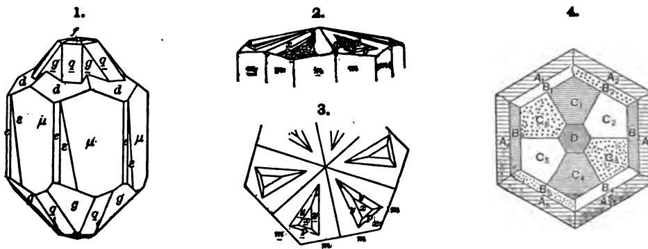
Figs. 1-3, Websky; 4, Klein.
