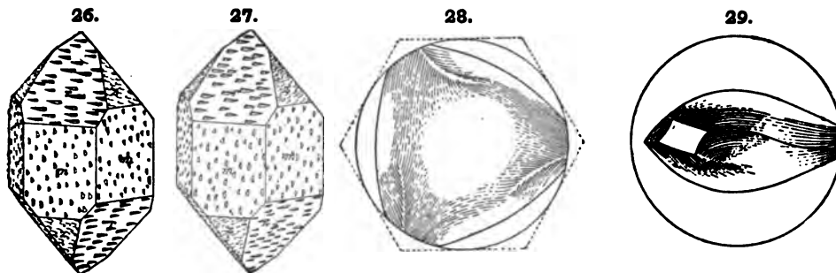
Figs. 26-29, Crystals etched by hydrofluoric acid, Penfield. 26, right-handed, 27, left-handed, crystal. 28, 29, sphere cut from simple right-handed crystal after being etched by acid for 7 weeks: 28, basal view; 29, front view; circle shows original form of sphere, dotted hexagon the position of axes.
