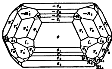
3, 4. Mte. Somma, Rath.
