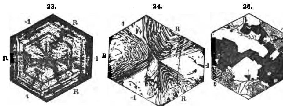
Figs. 23, 24, Basal sections in polarized light, showing interpenetration of right- and left-handed portions, Dx. 25. Same, showing also secondary lamellæ (at a , b ), alternately right- and left-handed, Judd.
