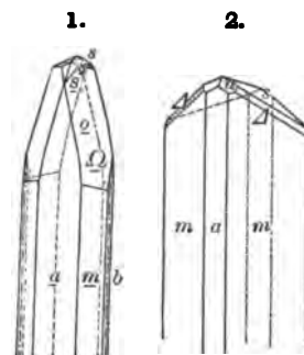
1, Acmite ; 2, Ægirite , Norway, Brögger.
