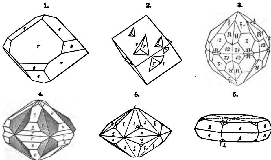
Figs. 1, 2, Common forms; 2, penetration-twin. 3, Färder, Tamrau. 4, Bohemia, Sbk. 5, 6, Phacolite, Richmond, Victoria, Rath.
