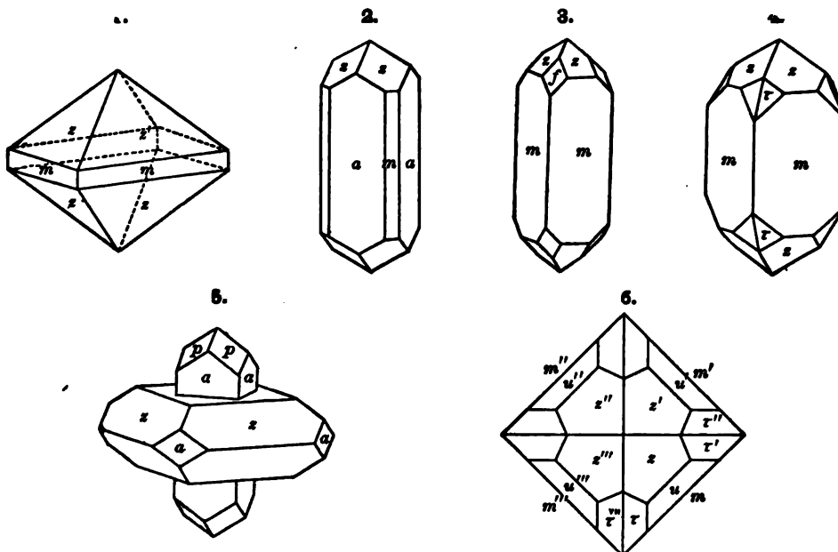
Fig. 1, Clarksville, Ga. 2, Binnenthal, Klein. 3, Alexander Co., N. C., Hidden. 4, Fibla, Klein. 5, Xenotime, enclosing zircon in parallel position, Henderson Co., N. C., Hidden. 6, Hitterö, after Flink
