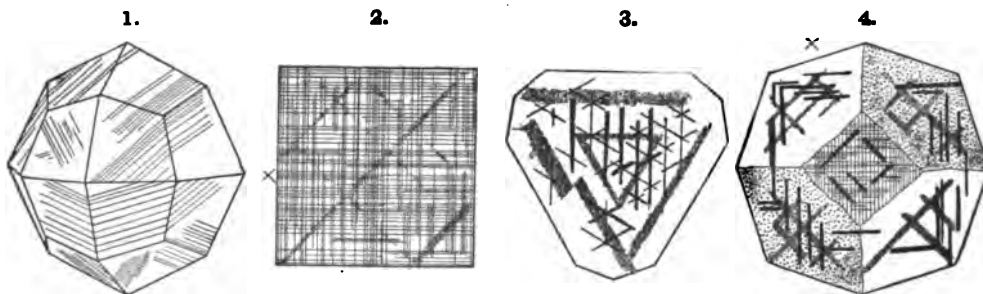
1, Common form, with twinning striations, Rath. 2-4, Sections, showing twinning lamellæ, as seen in polarized light, Klein: 2, section \parallel 001, showing fine tw. lamellæ \parallel 110, also others less numerous and sharp, parallel to two other dodecahedral faces; 3, section \parallel 111, with tw. lamellæ; 4, \parallel cubic face, composite crystal, of three individuals, cf. f. 2.
