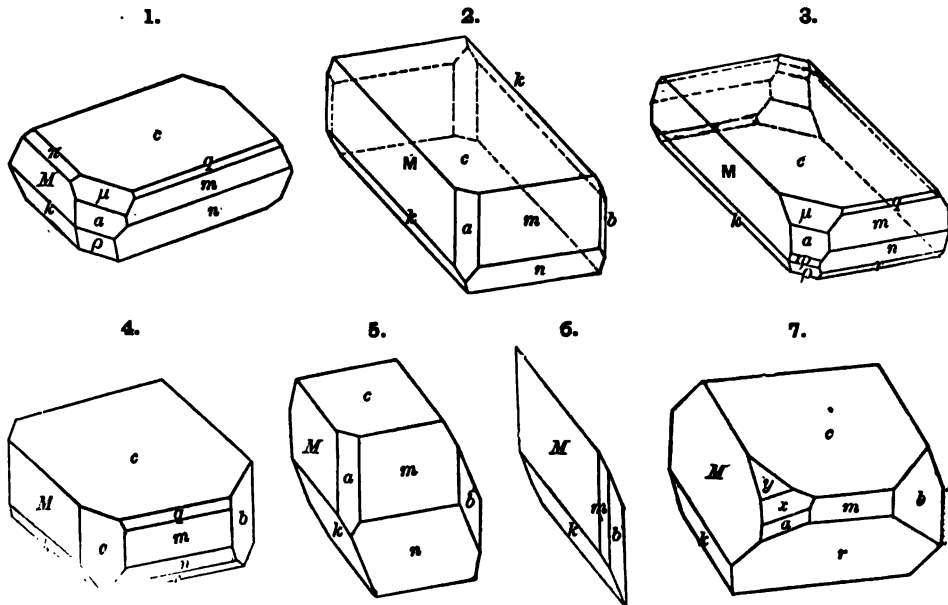
Figs. 1-4, Franklin Furnace, N. J. 2, 3, Pirsson. 5-7, Pajsberg, Flink.
