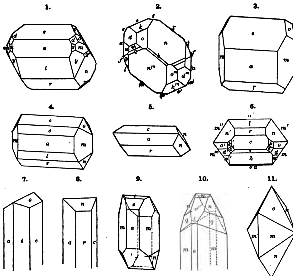
Figs. 1, Arendal, Hald. 2, Sulzbach, Bkg., projection on b (010). 3, Ural, Kk. 4, Achmatovsk, Kk. 5, Achmatovsk, after Kk., projection on plane \perp c . 6, 7, 8, common forms; 7, 8, with axis \perp b erect. 9, Elba, Artini. 10, Colorado, Bodewig. 11, Bucklandite , Achmatovsk, Kk.
