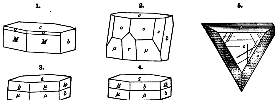
Figs. 1-5, Tschermak: 1, 2, Verneuil, simple crystals; 3, 4, twins; 5, Greenwood Furnace, parting forms with the gliding-planes \rho (205), \zeta (185).
