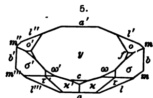
Wolframite , Sierra Almagrera, after Slg.
