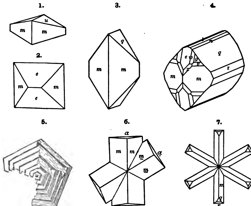
1, 3, Common forms. 2, Schladming, Rumpf. 4, Danaite , Franconia. 5, Deloro. 6, Servia Schmidt. 7, Weller, Bkg. 6
