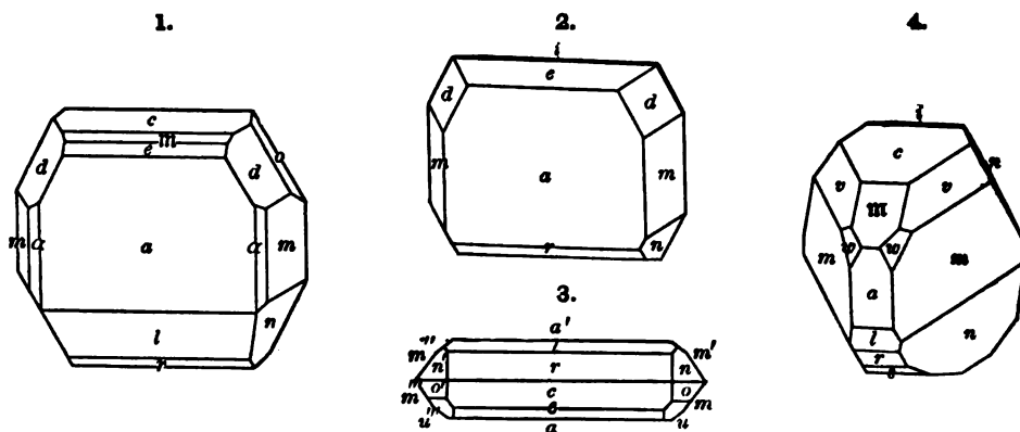
Figs. 1, Moriah, N. Y., \frac{1}{2} nat. size. 2, Uralorthite , Ilmen Mts., Kk. 3, Bucklandite , Laacher See, Rath. 4, Bagrathonite , Kk.
