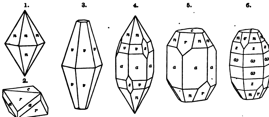
1, Ceylon. 2, Burma, Mallet. 3, Zánská, Id. 4, 5, Ceylon, Haid. 6, Ilmen Mts., Kk.
