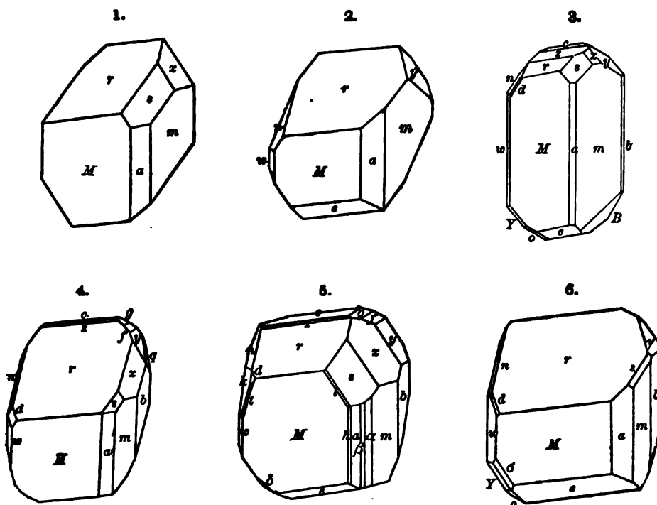
Figs. 1, Bourg d'Oisans. 2, Poloma, Schrauf. 3, Bethlehem, Penn., Frazier. 4, Botallack, Rath. 5, Bourg d'Oisans, Rath. 6, Poloma, Schrauf.
