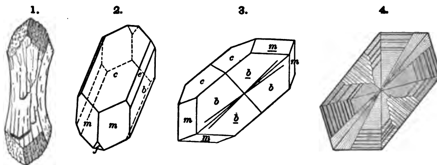
1, Sheaf-like crystal. 2-4, Lasaulx : 2, ideal simple crystal; 4, section \parallel b in polarized light.
