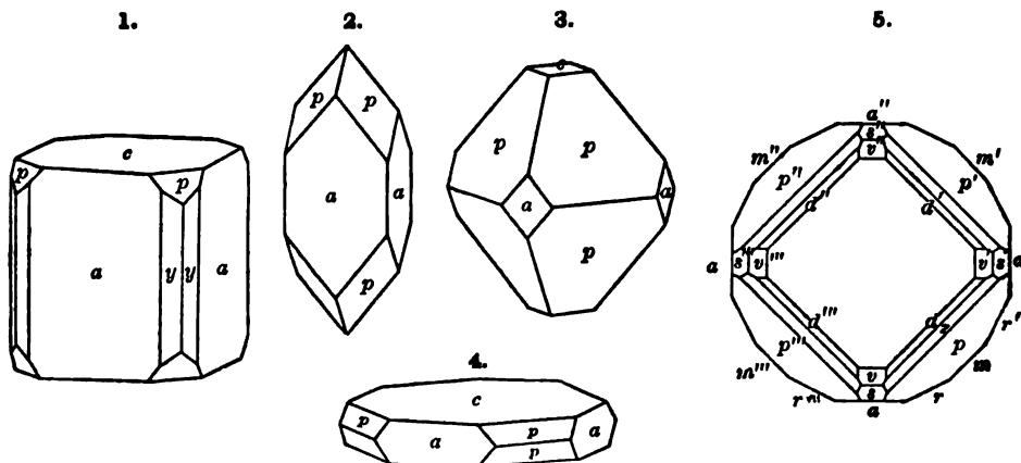
Figs. 1-8, Common forms. 4, L. Superior. 5, Utö, Sweden, after W. Müller .
