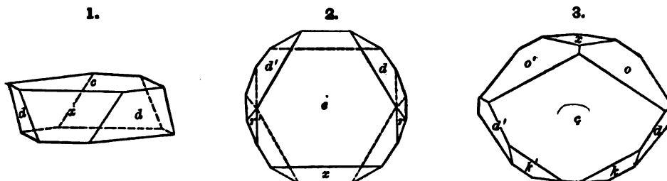
Figs. 1-3, Waluewite , Kk.: 2, with x (\bar{1}02) in front; 3, in normal position.
