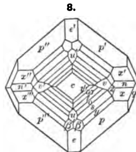
Rabbit Hole, Nev. 4
