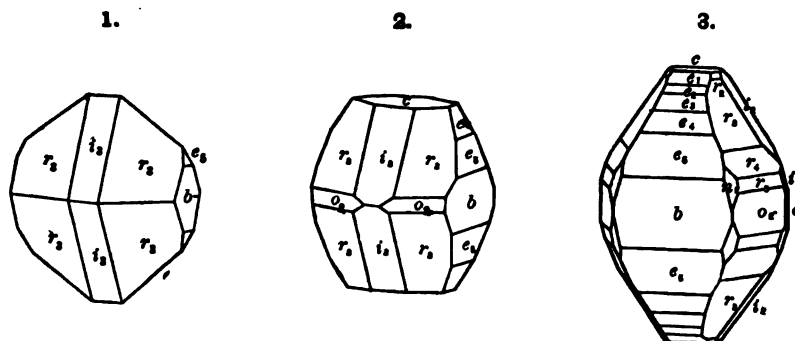
Figs. 1, 2, Ladu mine, Sweden, H. Sjögren. 3, 4, Monte Somma, Rath; drawn with b (010) in front.
