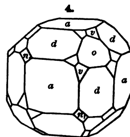
After Groth.
