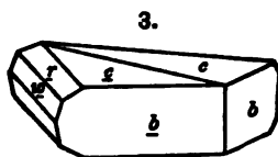
Frieselite, Vrba.
