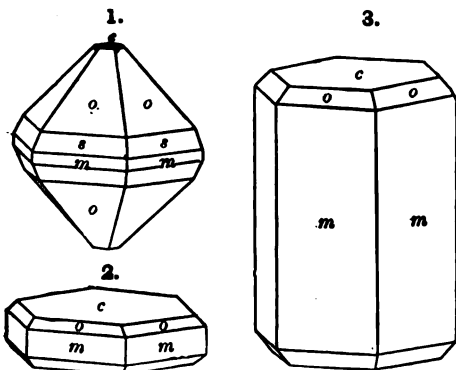
Figs. 1-3, Ayres.
