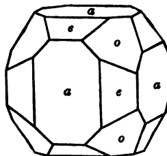
India, Mallet.
