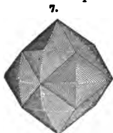
Heddle.
