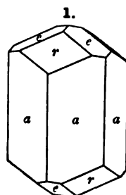
New Jersey.
