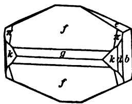
Virginia, Ayres.
