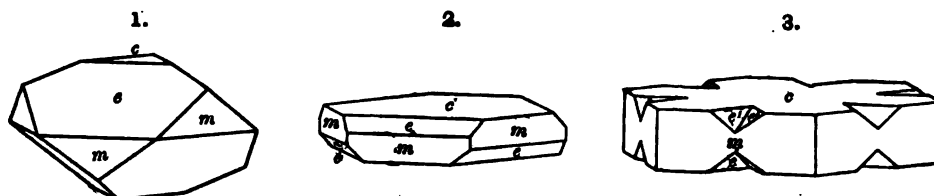
Figs. 1-3, Douglasshall, Bücking.
