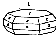
Ural, Rose.
