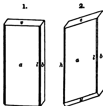
Norway, Brögger.
