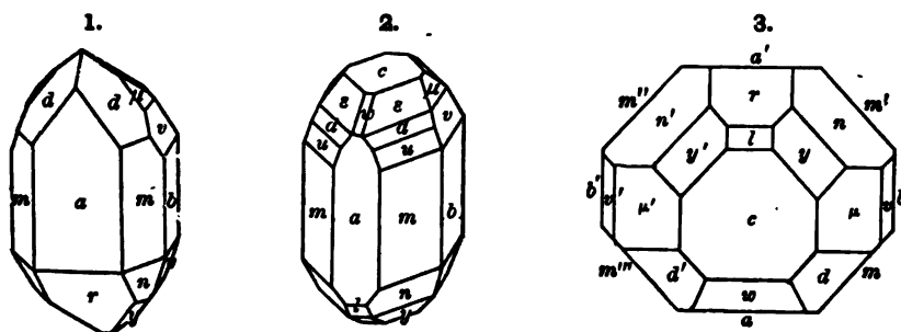
Figs. 1, 2, Aussee, Zepharovich.
