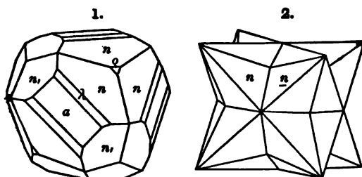
Figs. 1, 2, Schneeberg, Rath.
