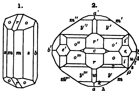
Figs. 1, 2, Elba; 2, Rath.
