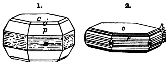
Figs. 1, 2, Penfield.
