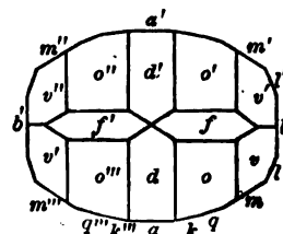
Tennessee.
