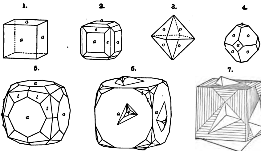
Figs. 1-4, simple forms.
