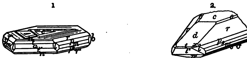
Figs. 1, 2, Marysvale, Montana.
