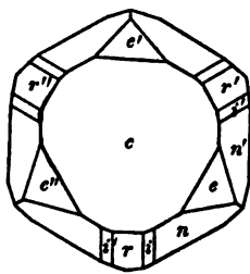
Ural, Kk.
