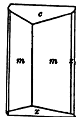
Binnenthal, Obermayer.
