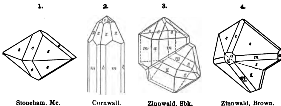
Stoneham, Me.
