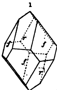
Hamlinite.
