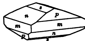
Haidinger.
