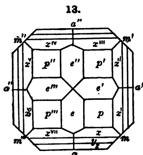
Sausalpe, after Haidinger.
