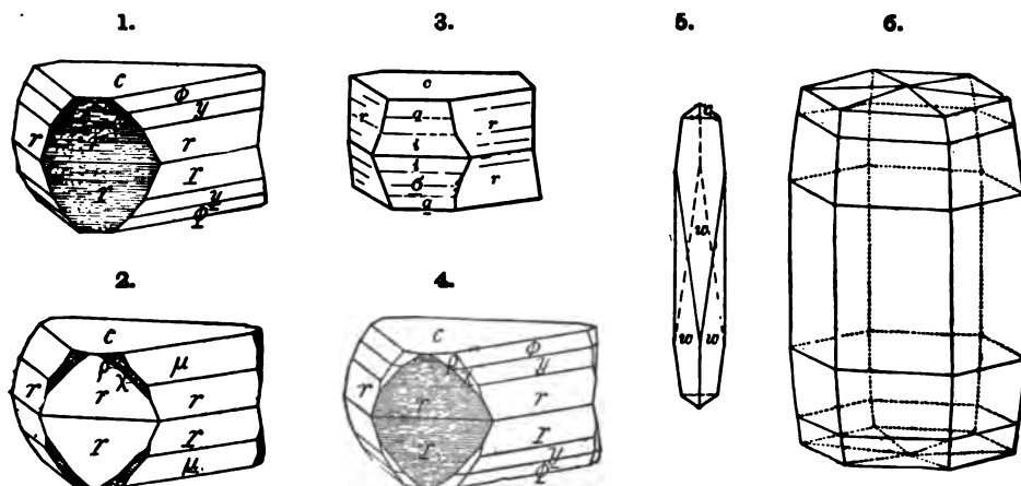
Figs. 1, 2, 4, Texas, Penn., Pirsson. 3, Zermatt, Tschermak. 5, Zillertal, Id. 6, Kämmererite, Kk.
