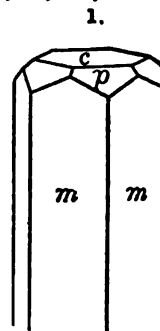
Penfieldite.
