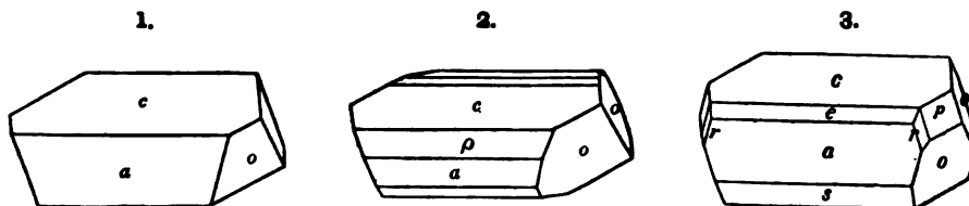
Figs. 1, 2, Zepharovich. 3, Ayres.
