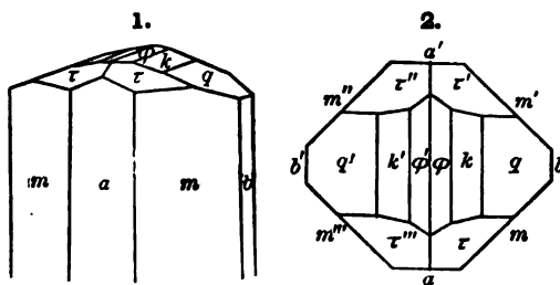
Figs. 1, 2, Bamle, Rath.
