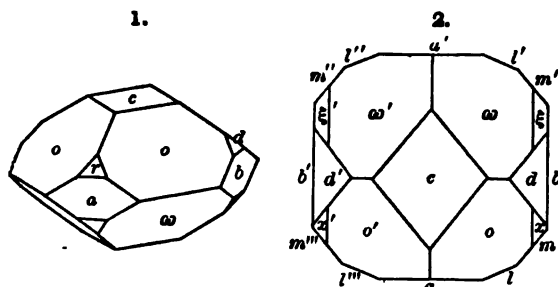
Figs. 1, 2, Loederburg, Luedecke.
