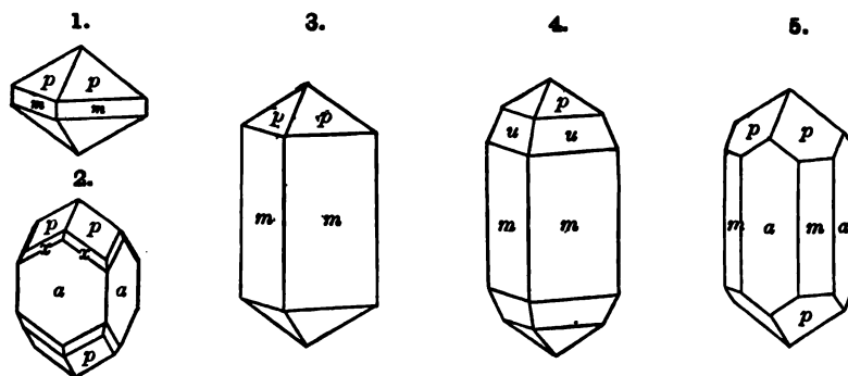
Figs. 1-5, Common forms.
