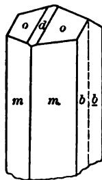
Iceland, Flink.
