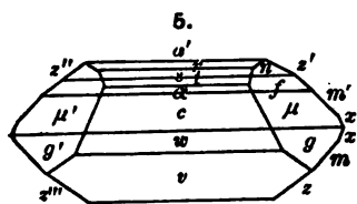
Vesuvius, Rath.
