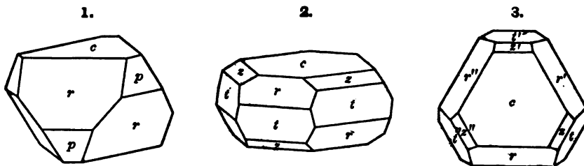
Fig. 1, Low's Mine, Texas, Penn.
