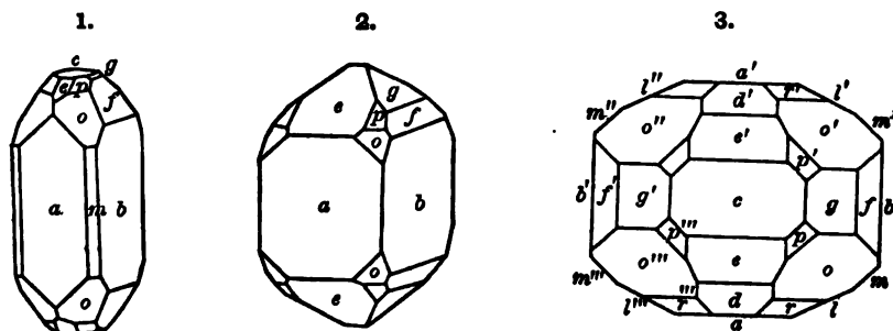
Figs. 1-3, after Schmidt.
