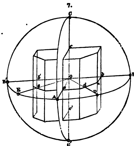
After Brezina.
