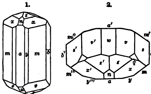
Figs. 1, 2, Cornwall. Rath.
