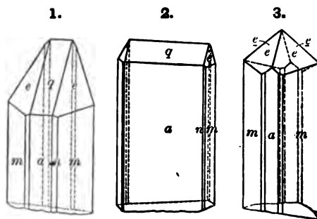
Figs. 1-3, Norway, Bgr.
