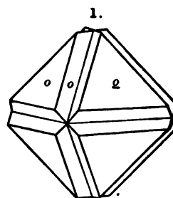
Albano, Rath.
