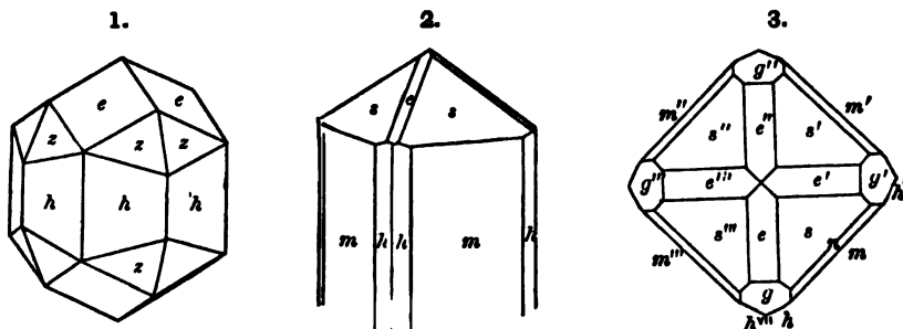
Figs. 1–3, Platten, Bohemia.
