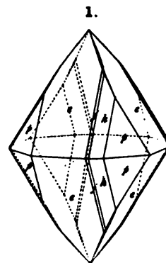
Powellite.
