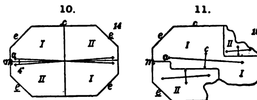
Stoneham.
