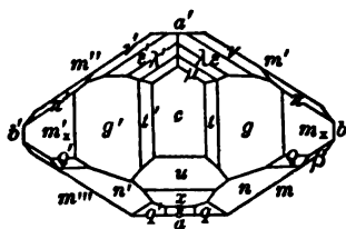
Bergen Hill.
