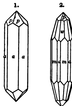
Figs. 1, 2, Cornwall, Maskelyne.
