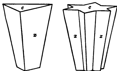
Pfibrum, Zeph.
