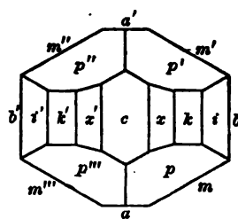
After Mr.
