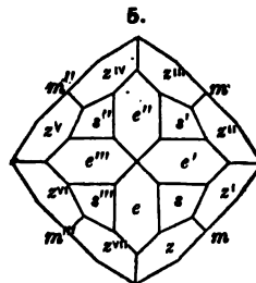
Cornwall, Haid.
