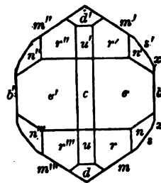
Chili, Brögger.
