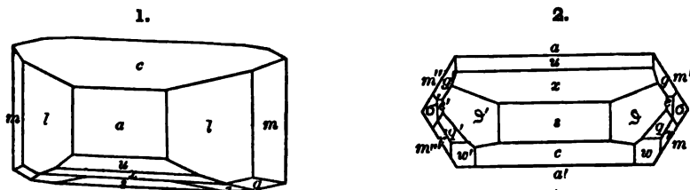
Figs. 1, 2, After Koksharov.
