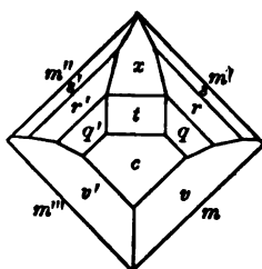
Greenland, Knr.
