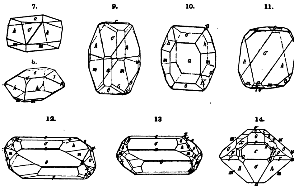
7-14, Arizona, Farrington.
