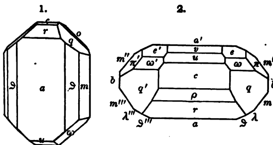
Fig. 1, 2. After Rumpf.
