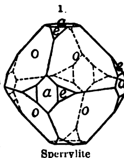
Sperrylite
