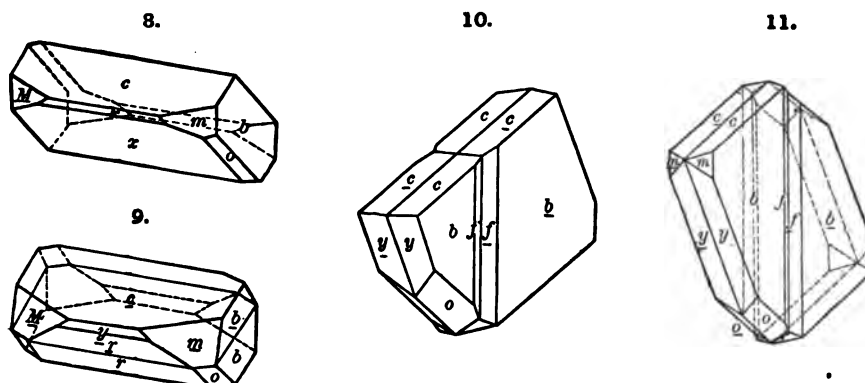
8, 9, Pericline, Schrauf. 10, 11, Roe Tourné, Savoy, Rose.
