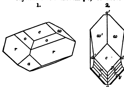
Figs. Wolfsberg; 1, Rose; 2, after Luedecke.
