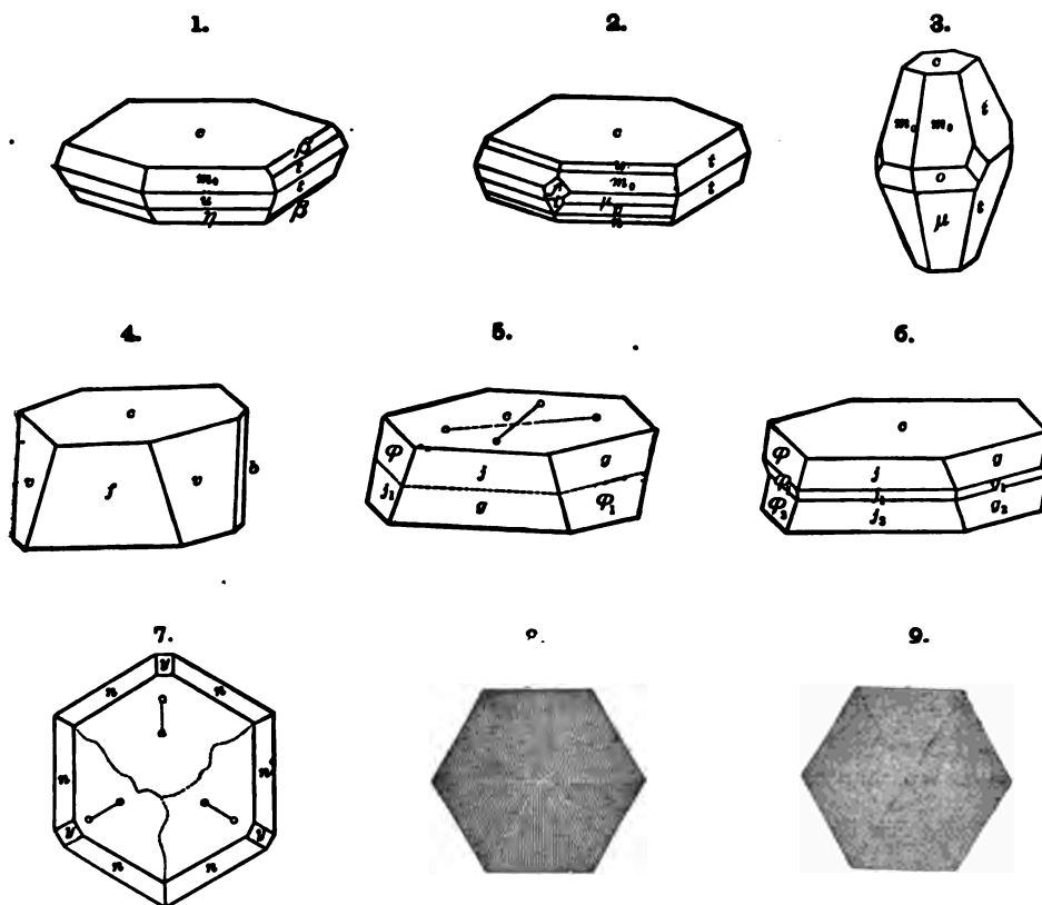
Figs. 1-7, Tschermak: 1, Pfätsch; 2, 8, Achmatovsk; 4, Schwarzenstein (Hbg.); 5, Zillerthal, twin, mica law; 6, do., twin, penninite law; 7, Achmatovsk, trilling. 8, 9, J. P. Cooke: 8, West Chester; 9, Texas.
