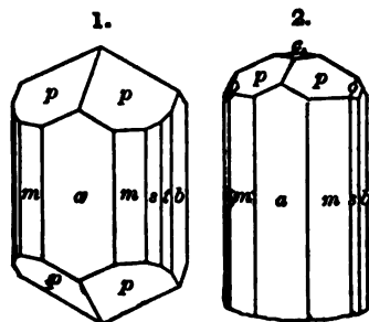
Figs. 1, 2, Norway; 1, Rose; 2, Bgr.
